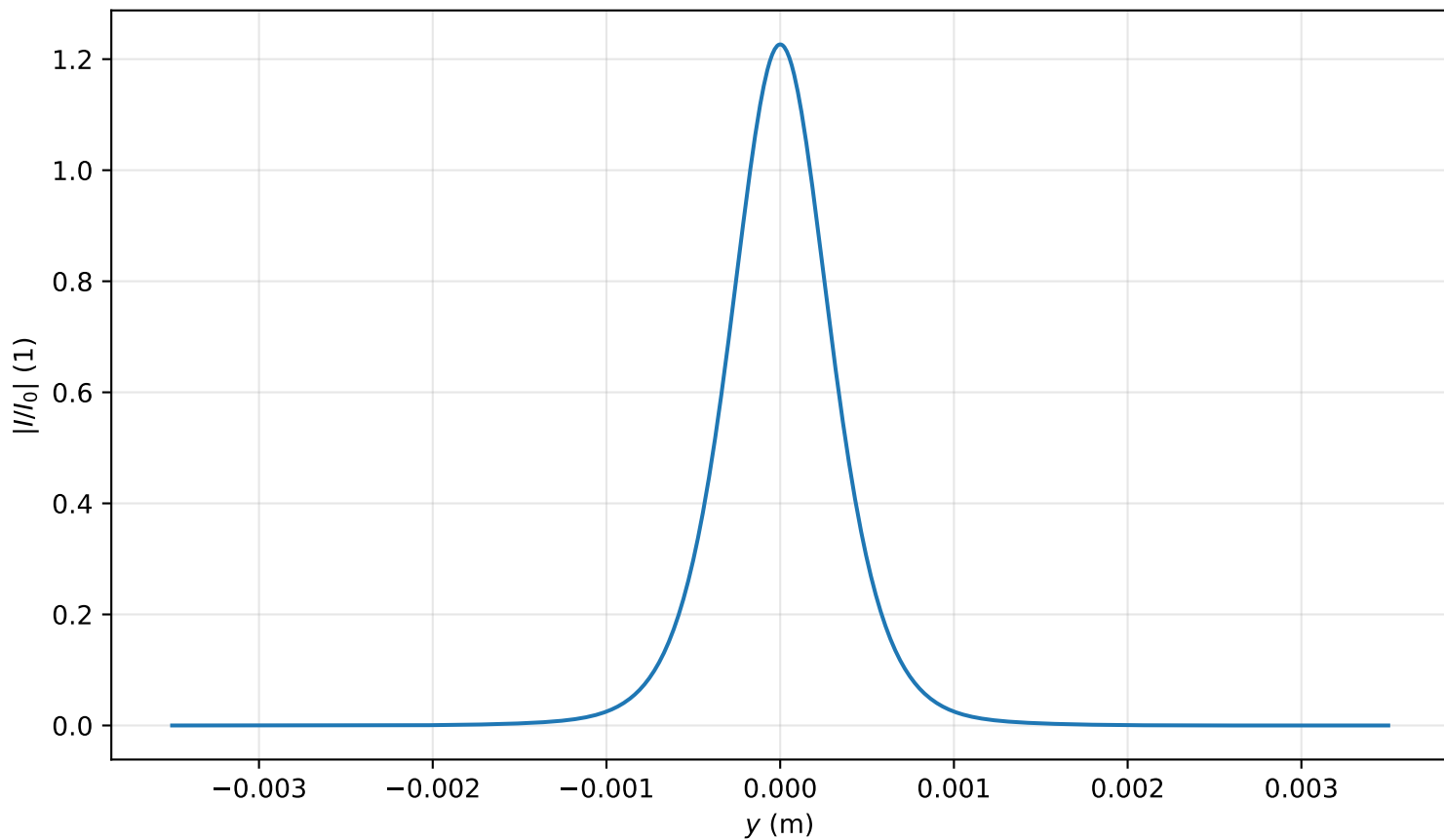
Intensity profile I(x=0, y, z=2.468)/I_0 , P_{in}=0.8P_{cr} , artificial time
